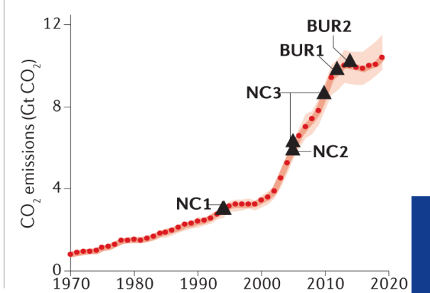
d CO 2 emissions trend in China
